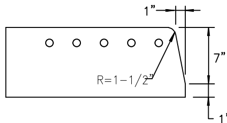
CURB FACE DETAIL SECTION "B-B"
